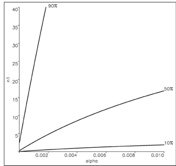
Figure 4. Number of class I CIN genes, n_1 , needed for a 10%, 50%, and 90% probability that CIN emerges before the inactivation of APC , in dependence of the probability \alpha that a cell with two inactivated APC alleles, APC -/- , sticks on top of the crypt and initiates dysplastic growth. Parameter values are N = 1000 , \tau_0 = 1 , \tau_1 = 1 , q = 0.01 , and t = 70 years.
